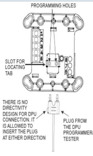
Model XTRI-D | XTRI-R | XTRI-S Intelligent Device Interface Module
