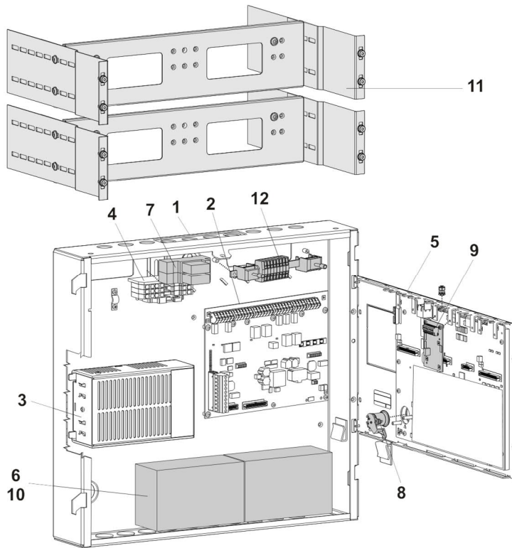
Fig. 2: Layout of FC721
