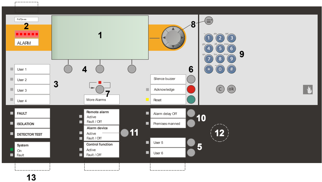
Fig. 4: Indication and operating elements
