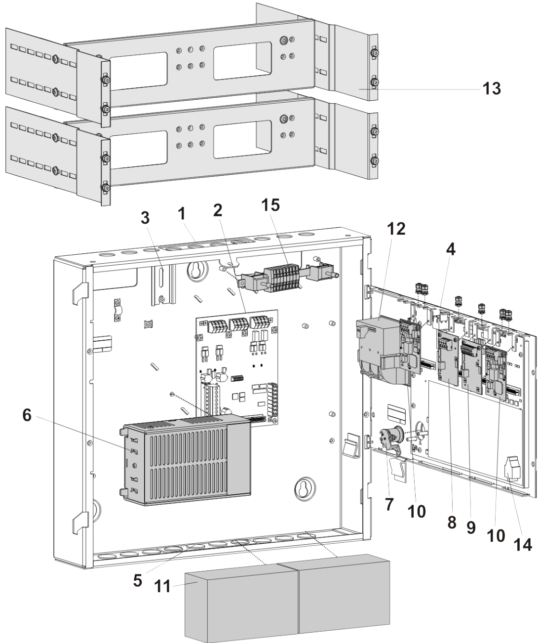
Fig. 5: Layout of FT724
